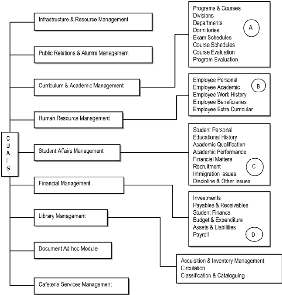
Figure A3-4. Partial UITC for the CUAIS Project
