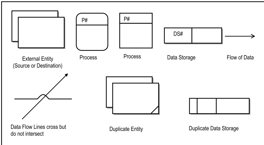
Figure 6-9. Symbols Used in DFD
