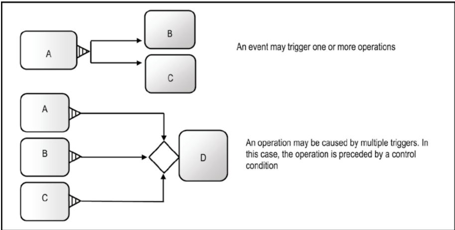
Figure A6-10. Illustrating the Relationship between Triggers and Operations
