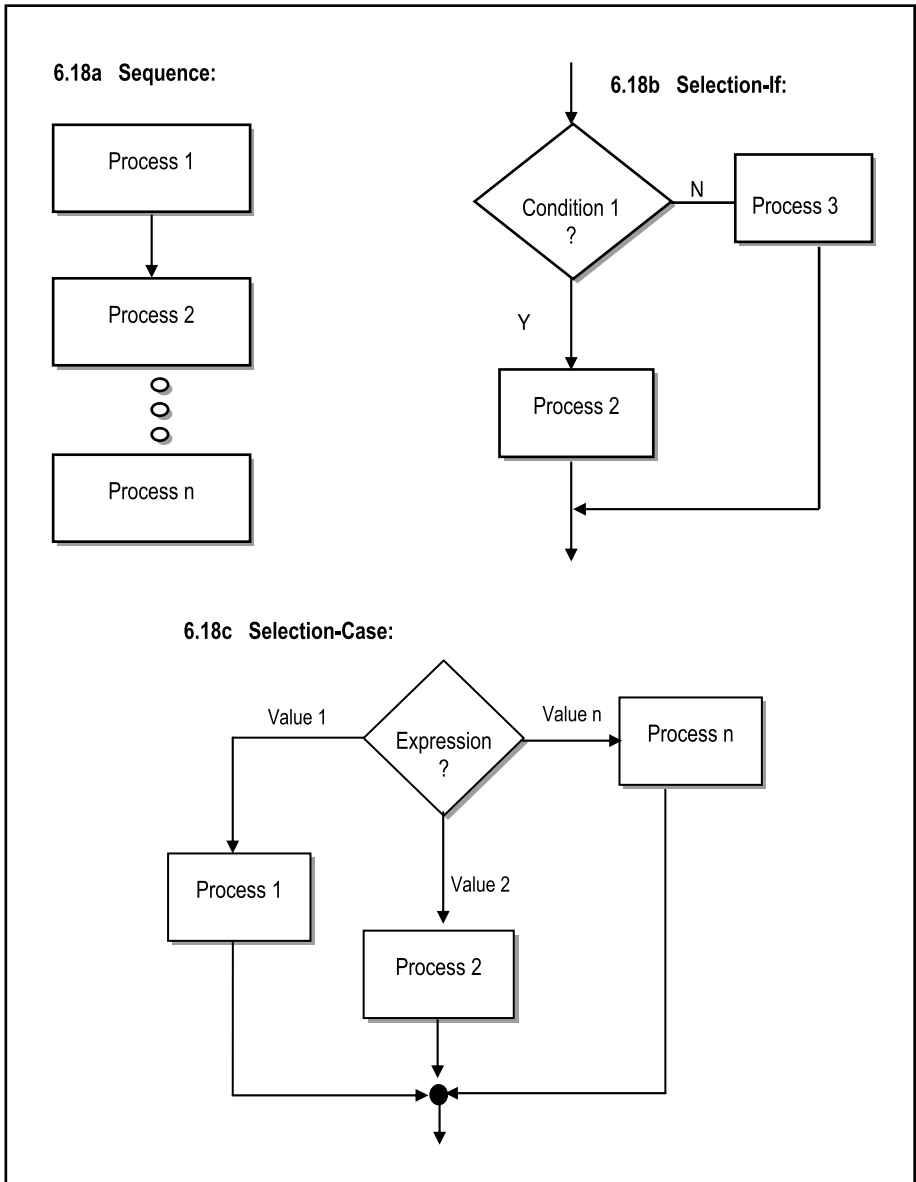
Figure 6-18. Control Structures for Program Flow Chart
