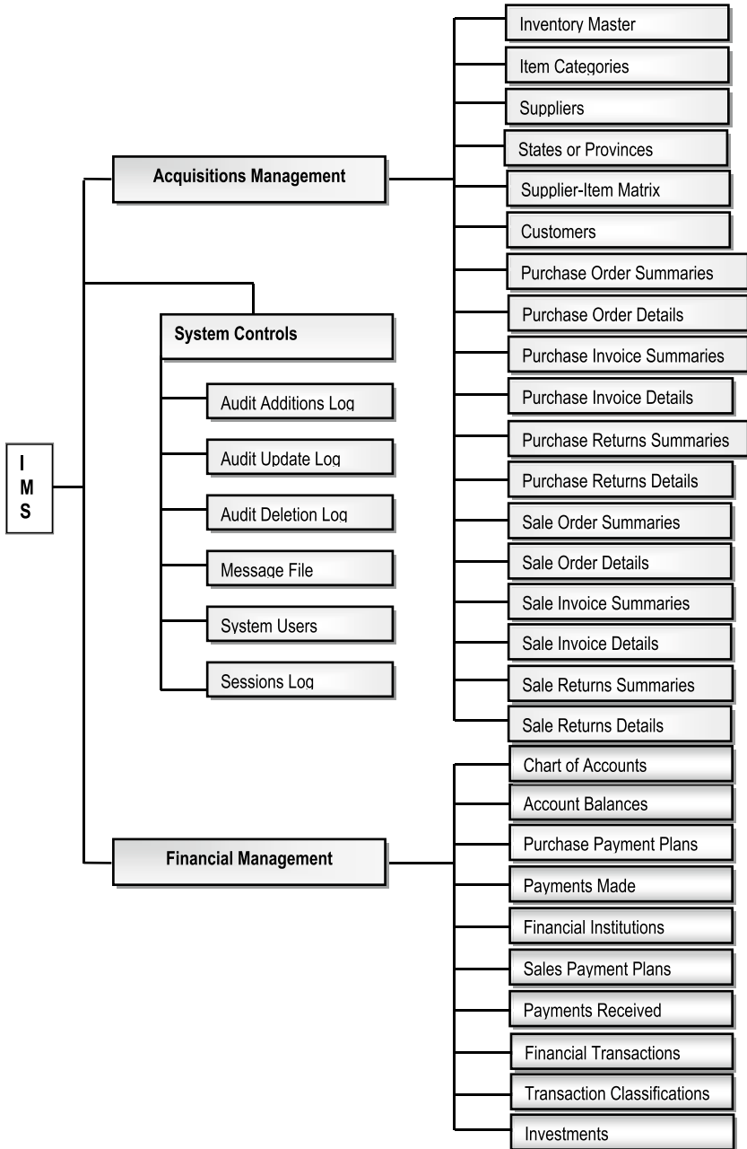
Figure A10-1. IMS Information Topology Chart
