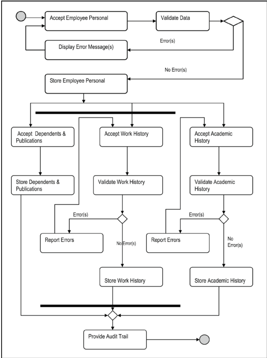
Figure A6-13. Activity Diagram for Adding Employee Information
