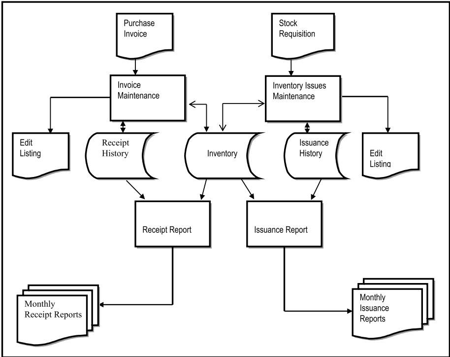
Figure 6-4. Process-Oriented Flowchart for (part of an) Inventory Management System
