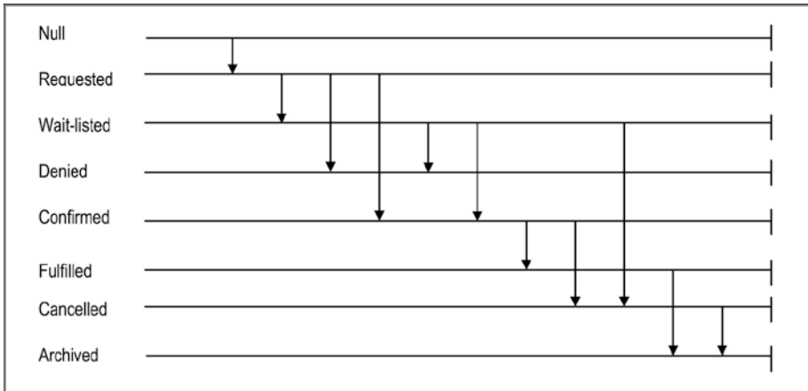
Figure A6-5. State Transition Diagram for Airline Booking Object
