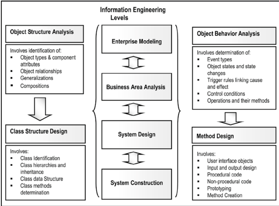
Figure A4-5. OO Modeling Hierarchy
