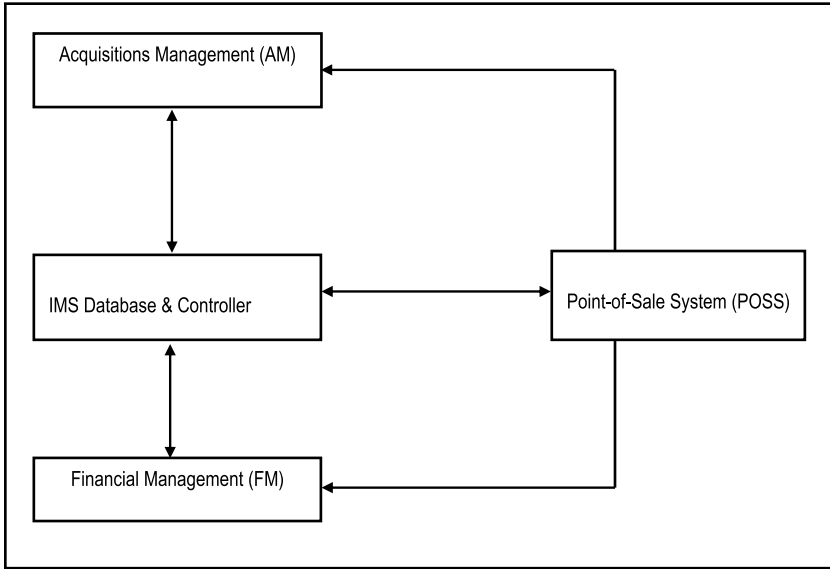
Figure A10-2. IMS Object Flow Diagram
