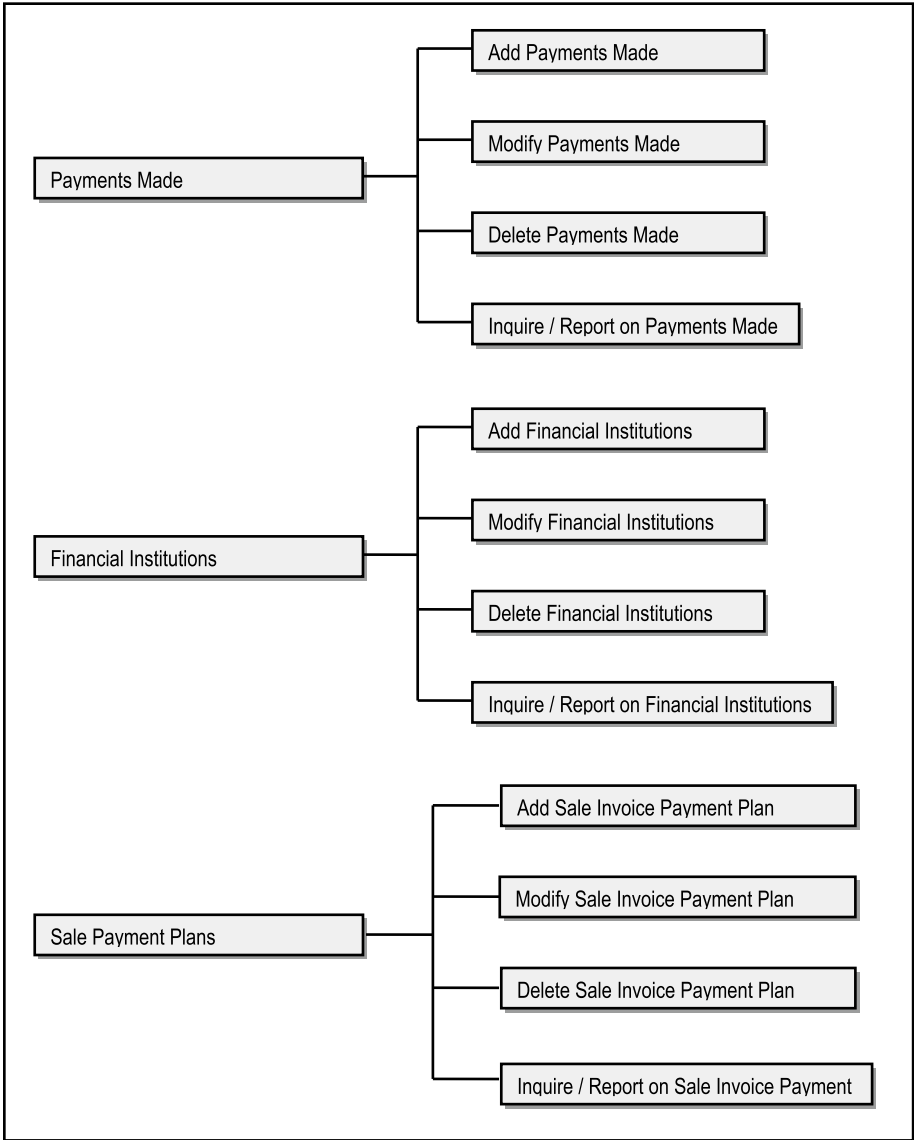
Figure A10-10. UITC for the IMS (continued)
