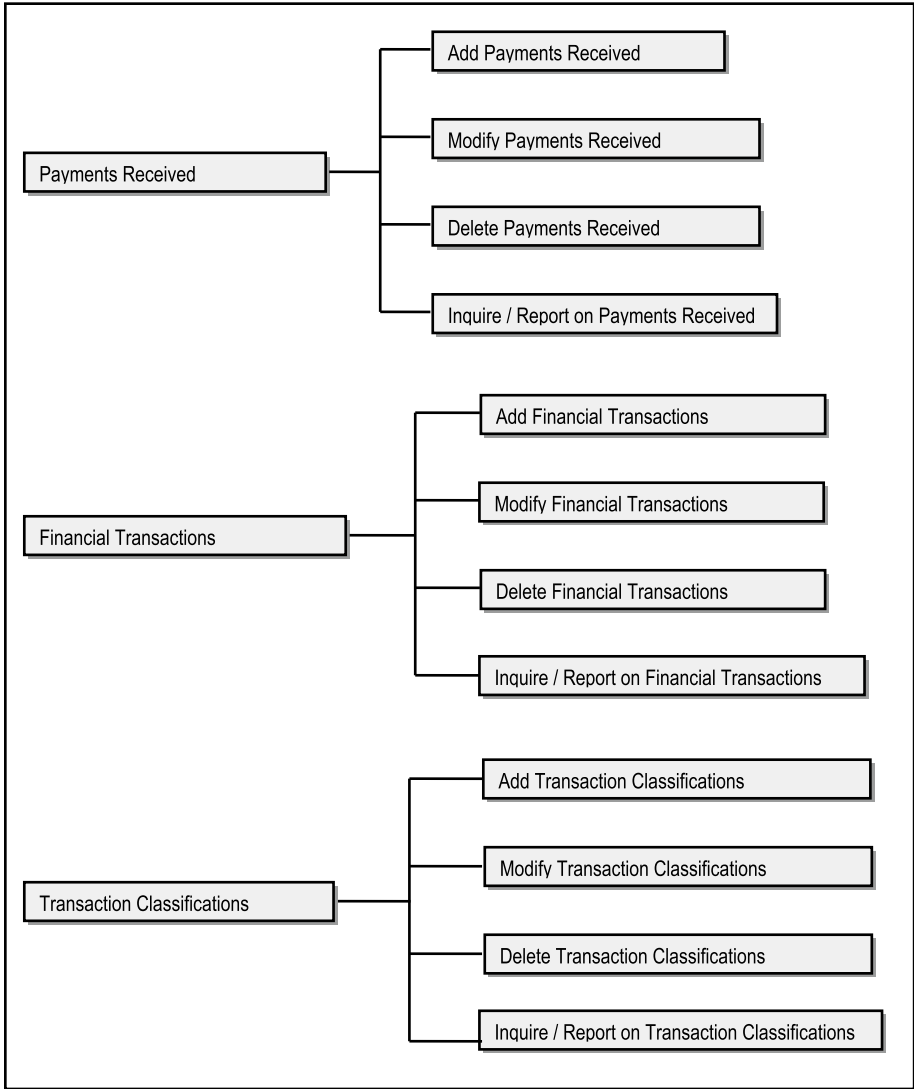
Figure A10-10. UITC for the IMS (continued)
