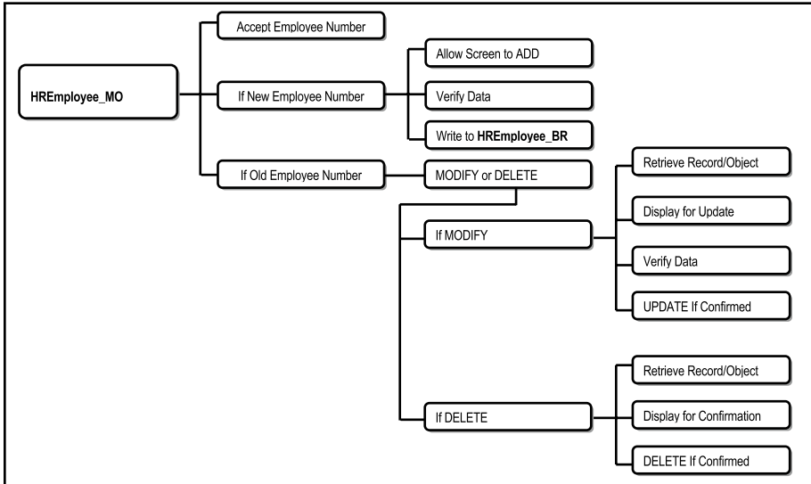
Figure 12-4. Warnier-Orr Diagram for a MAINTAIN Operation
