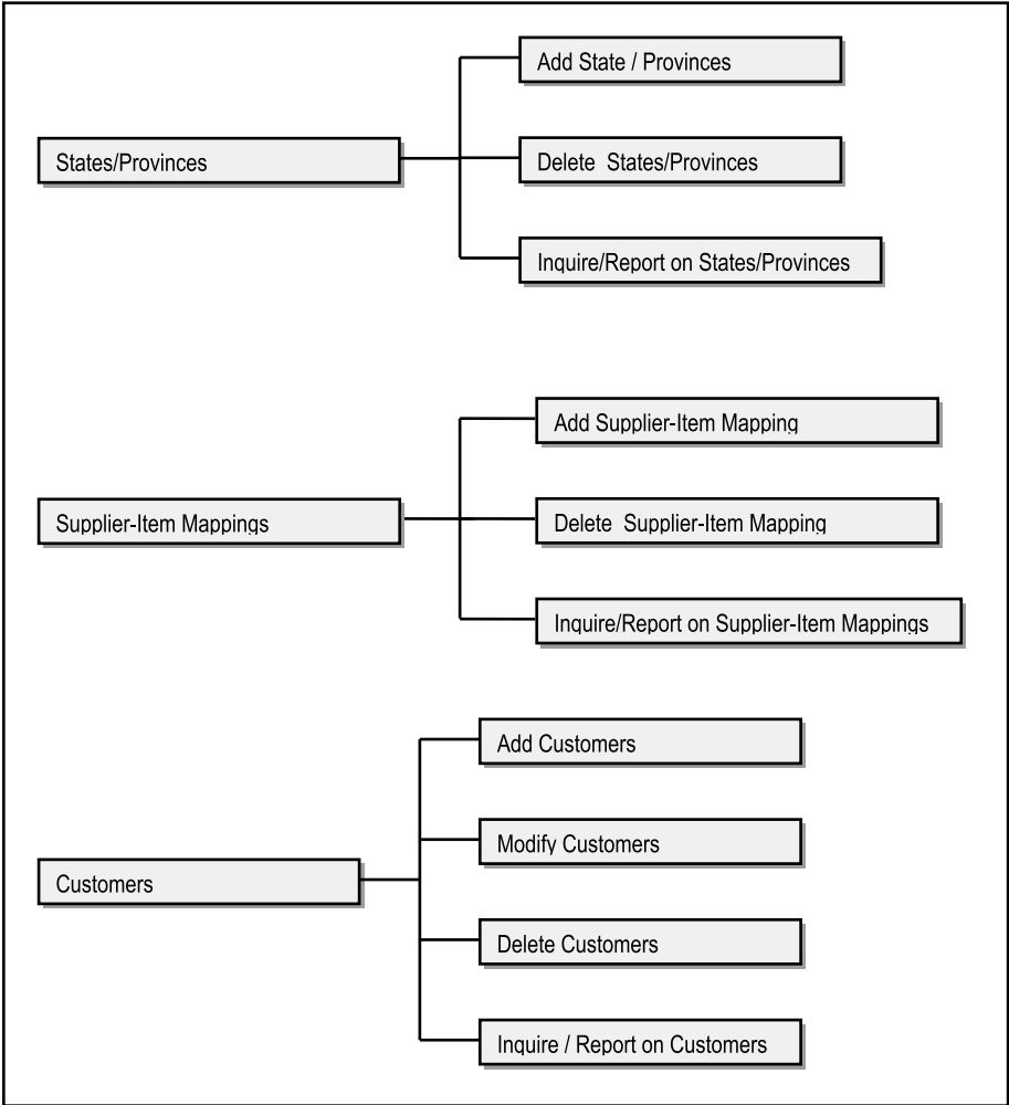
Figure A10-10. UITC for the IMS (continued)
