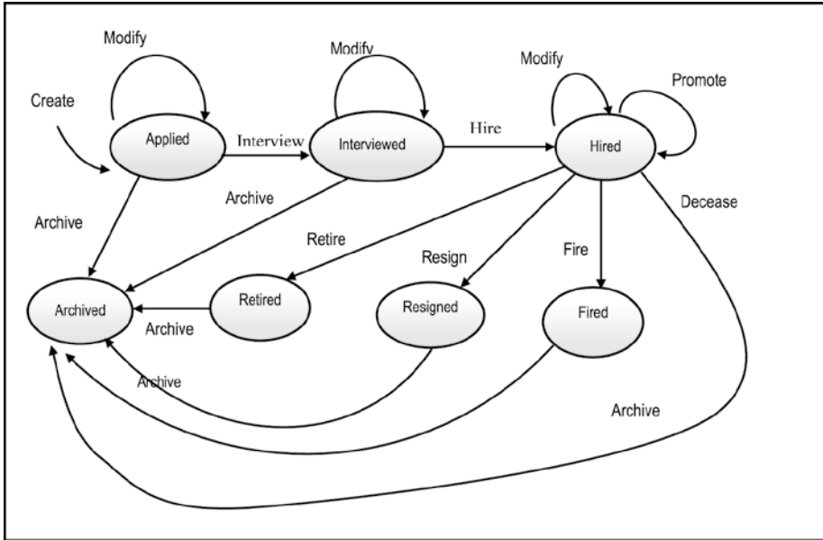
Figure A6-6. FSM for Employee Object
