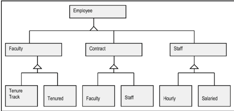
Figure A5-11. Multiple Inheritances via Nested Generalization
