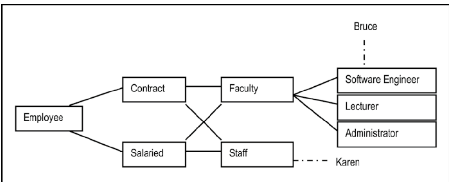
Figure A5-3. Fern Diagram with Instances
