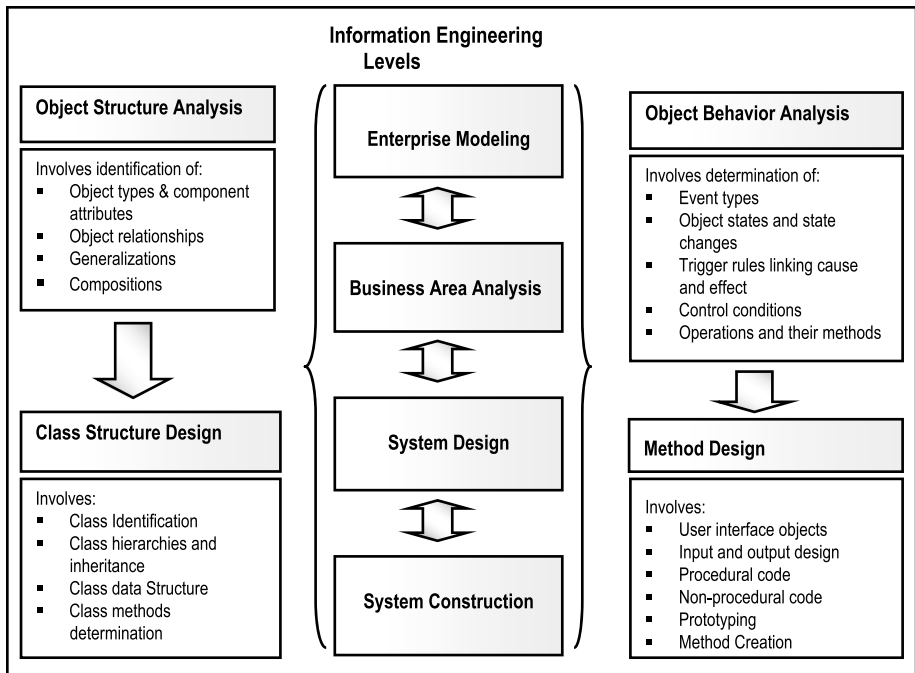
Figure 7-11. OO Modeling Pyramid
