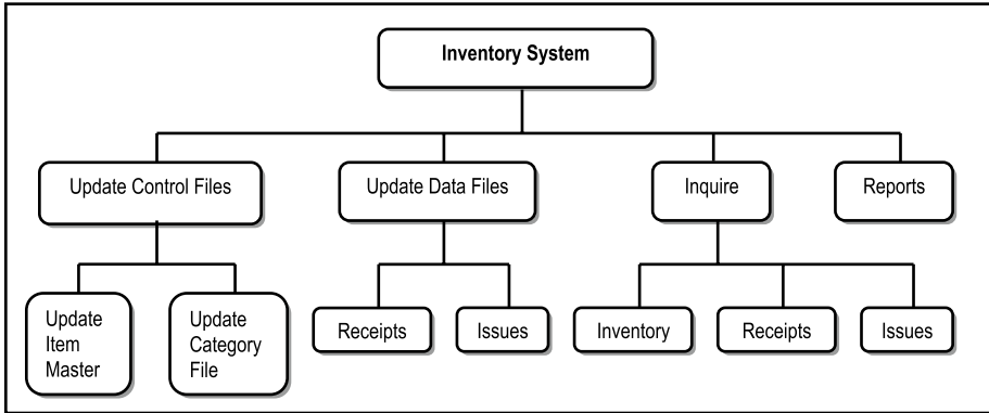
Figure 6-5a. Example of a HIPO Chart
