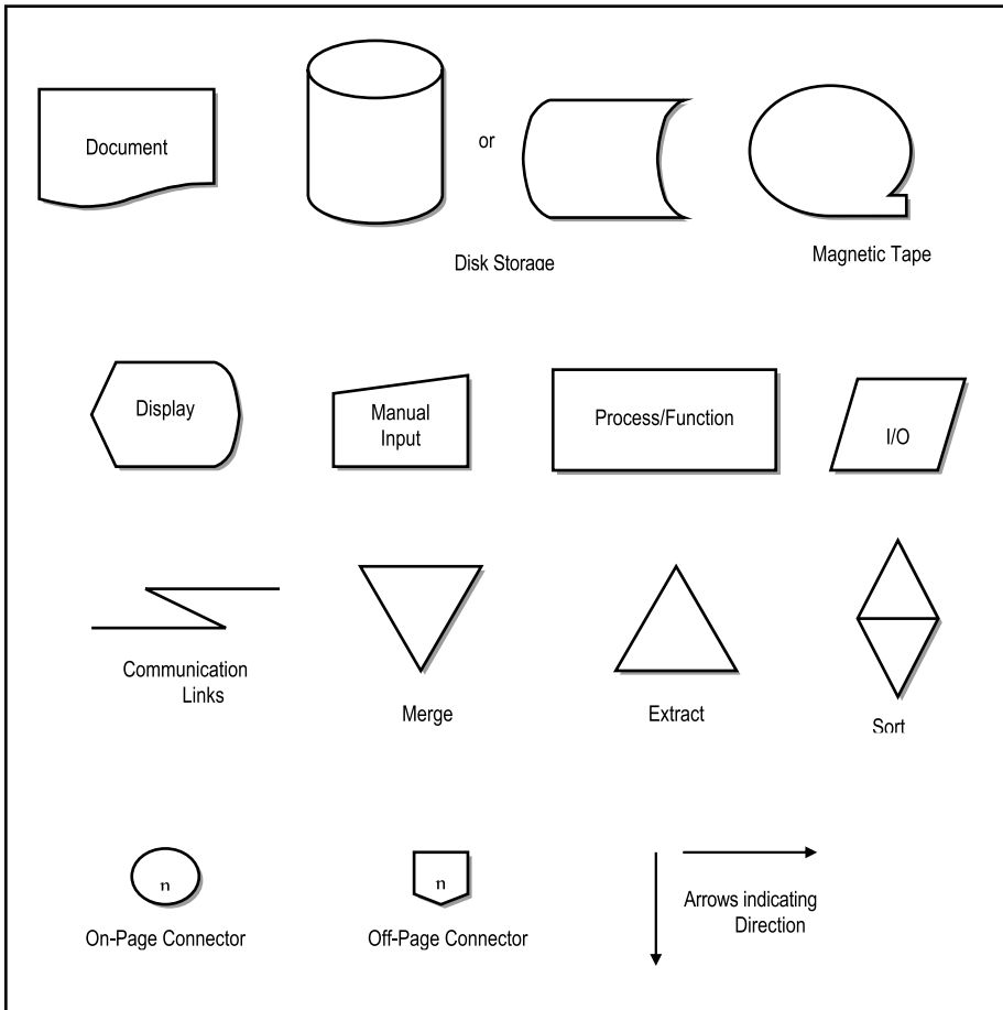
Figure 6-2. Traditional System Flowchart Symbols
