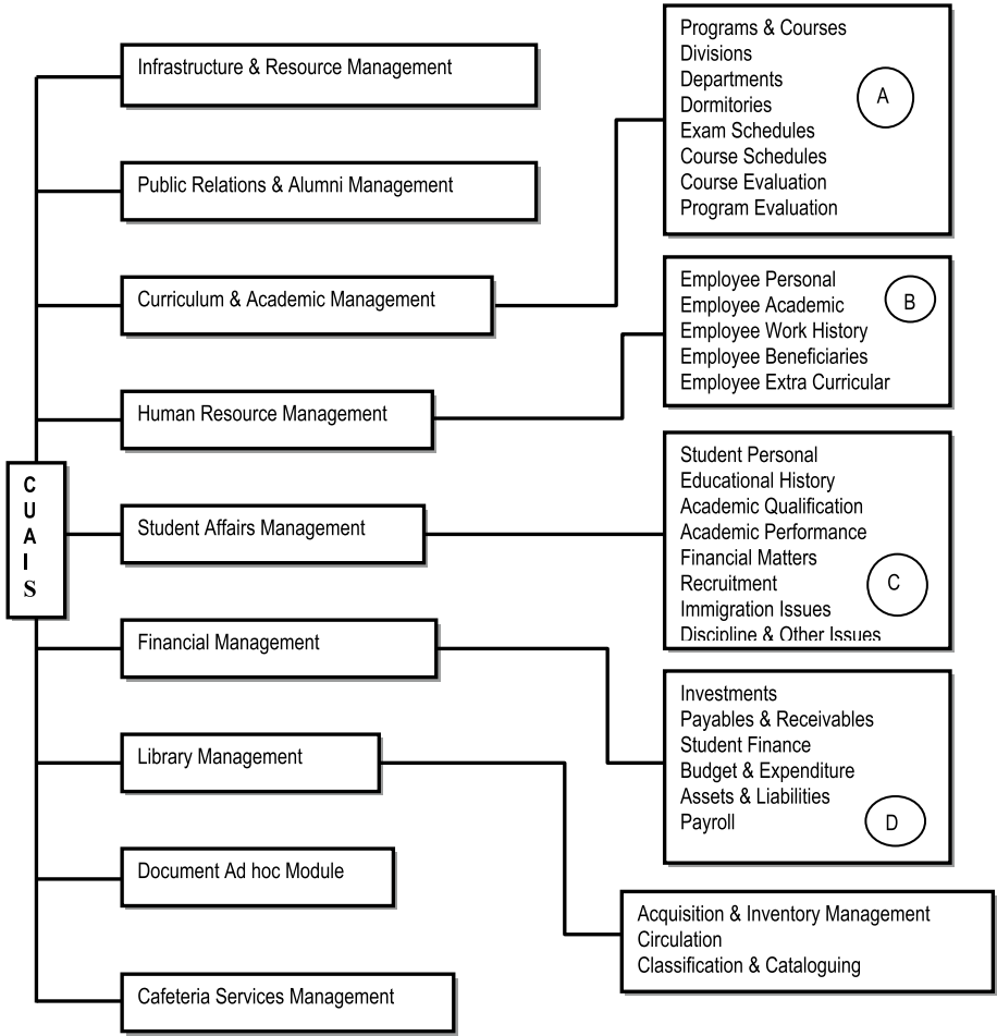
Figure 6-8. Partial User Interface Topology Chart for the CUAIS Project
