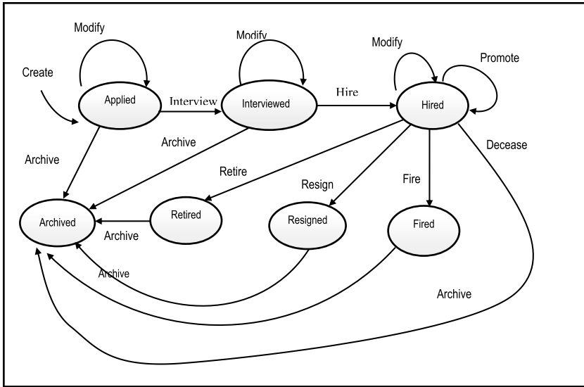
Figure 6-16. FSM for Employee
