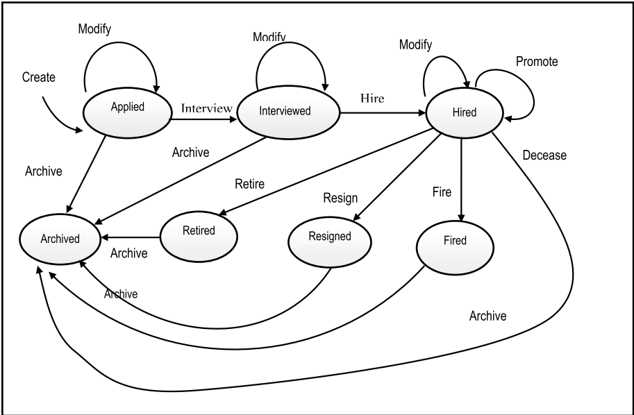
Figure 12-6. State Diagram for Employee Object
