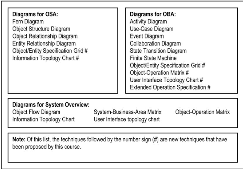
Figure A3-2. Recommended OOM Diagramming Techniques
