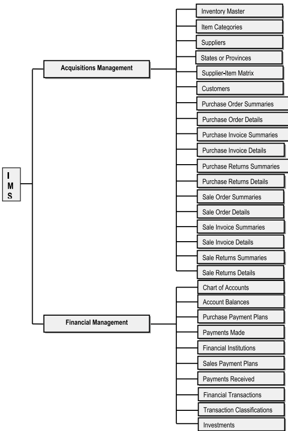
Figure A9-1. IMS Information Topology Chart
