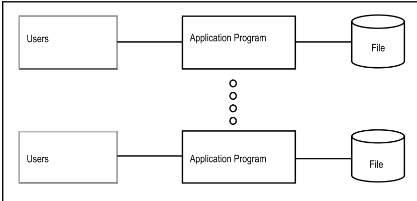
Figure 10-2. Conventional File-Based Design
