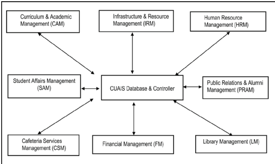
Figure A6-16. OFD for the CUAIS Project, Assuming Repository Model
