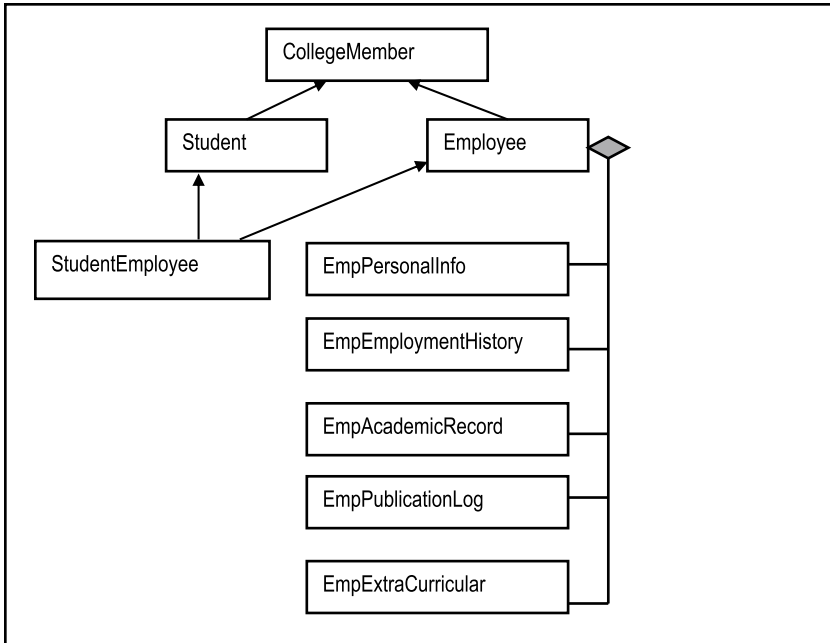
Figure 9-4. Abbreviated UML Diagram of an Inheritance Network for a College Community
