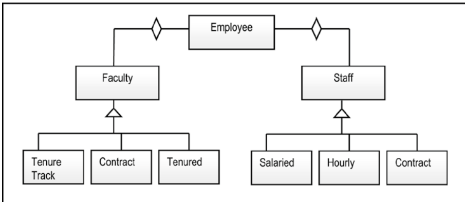
Figure A5-9. Multiple Inheritances using Delegation
