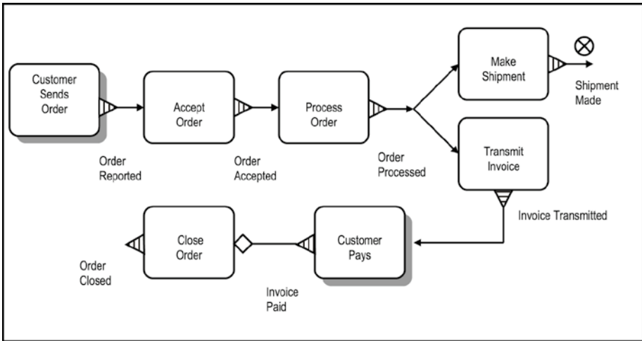
Figure A6-7. An Event Diagram for Processing a Purchase Order
