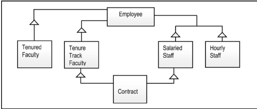
Figure A5-8. A Multiple Inheritance Problem
