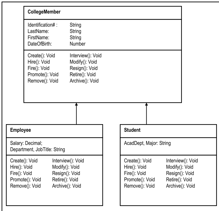
Figure 9-3. UML Diagram of a Type Hierarchy for a College Community
