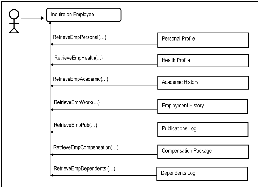
Figure 12-8. Collaboration Diagram for Inquiry on Employee Information
