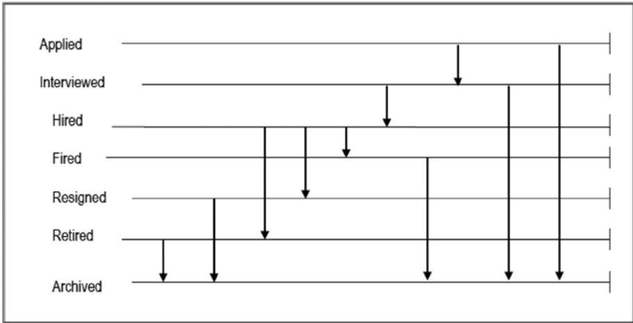
Figure A6-4. State Transition Diagram for Employee Object
