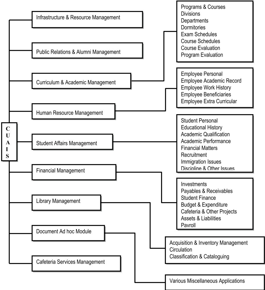
Figure A1-1. Information Topology Chart for the CUAIS Project
