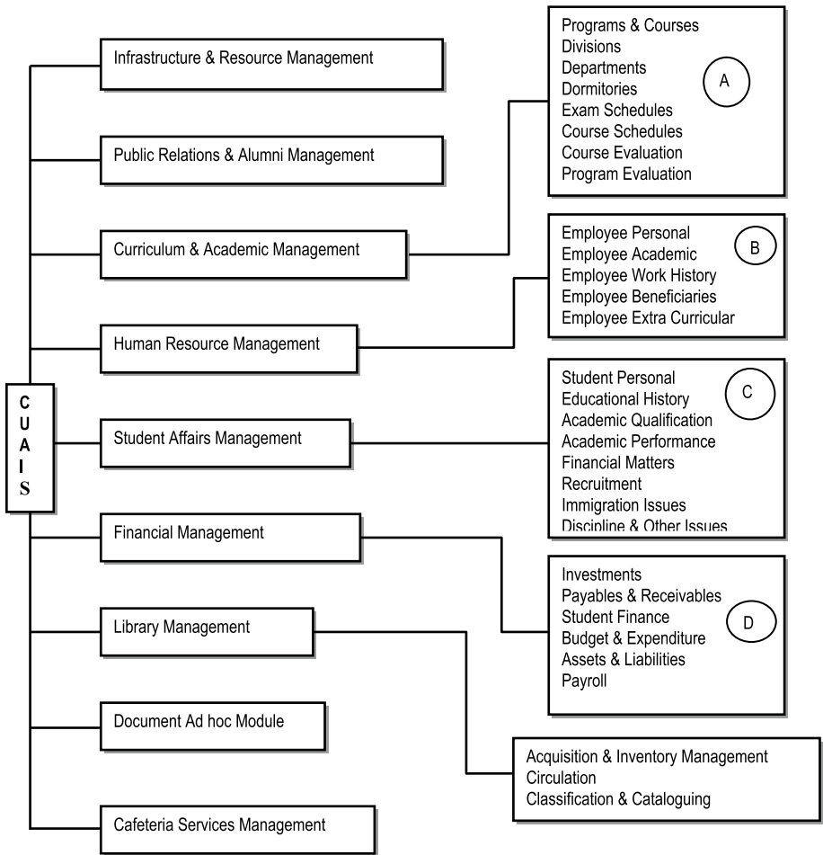
Figure 11-3. Partial UITC for the CUAIS Project
