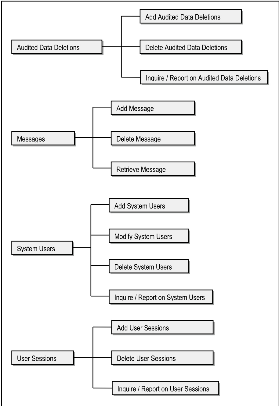
Figure A10-10. UITC for the IMS (continued)
