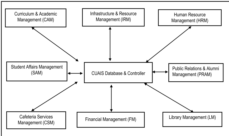
Figure 9-5. OFD for the CUAIS Project, Assuming Repository Model
