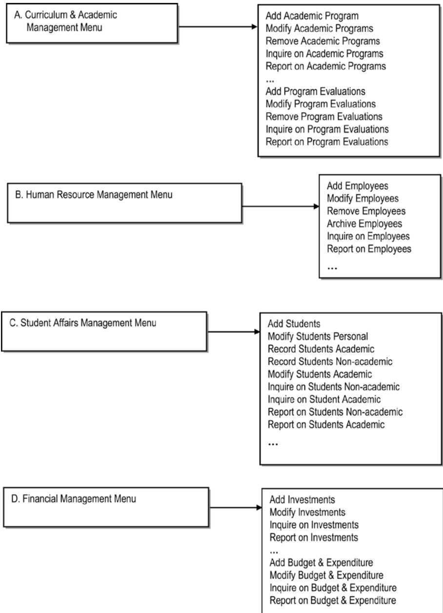
Figure A3-4. Partial UITC for the CUAIS Project (continued)
