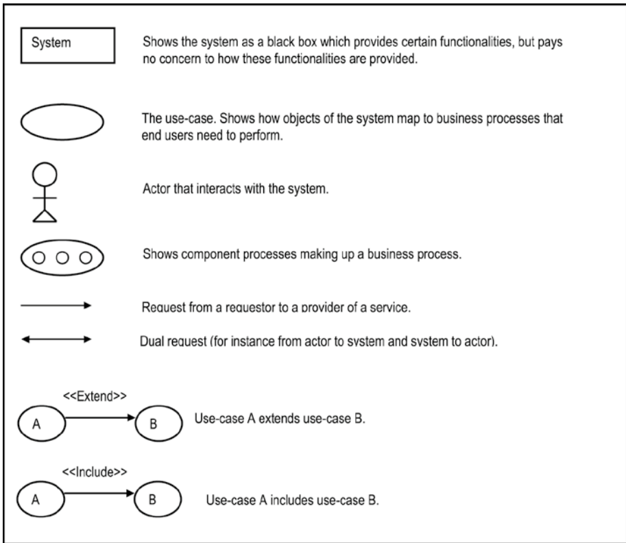
Figure A6-1. Symbols Used in Use-case Diagrams
