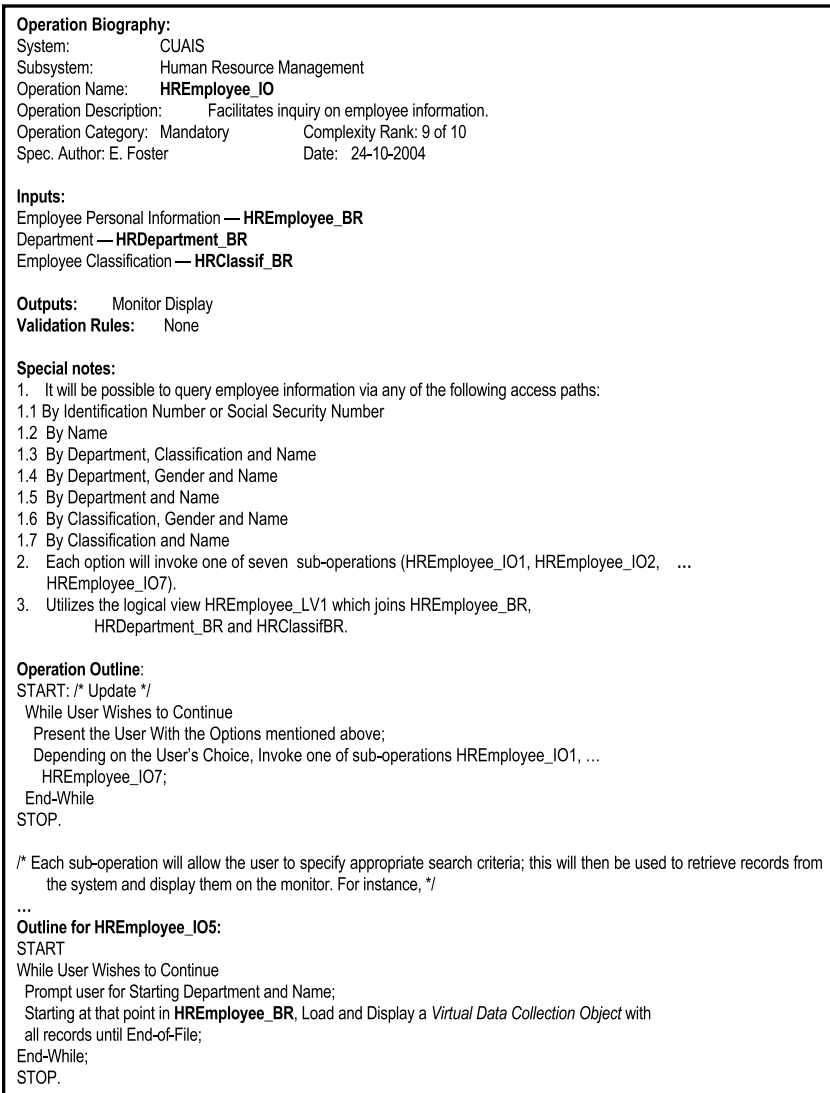
Figure 12-14. Sample EOS for INQUIRE Operation
