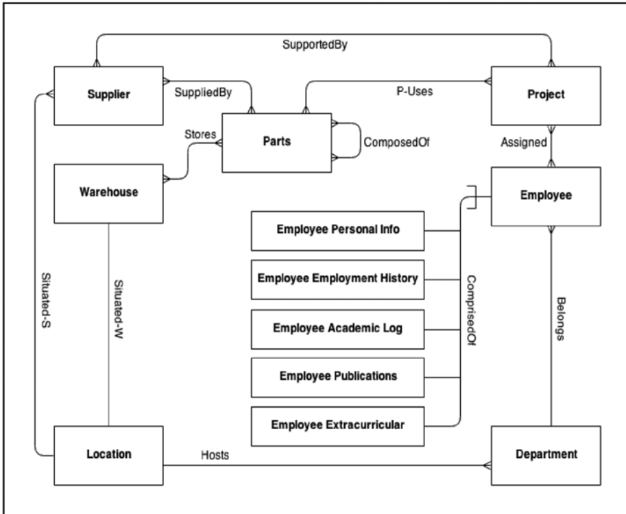
Figure 10-8. E-R Diagram for Manufacturing Environment
