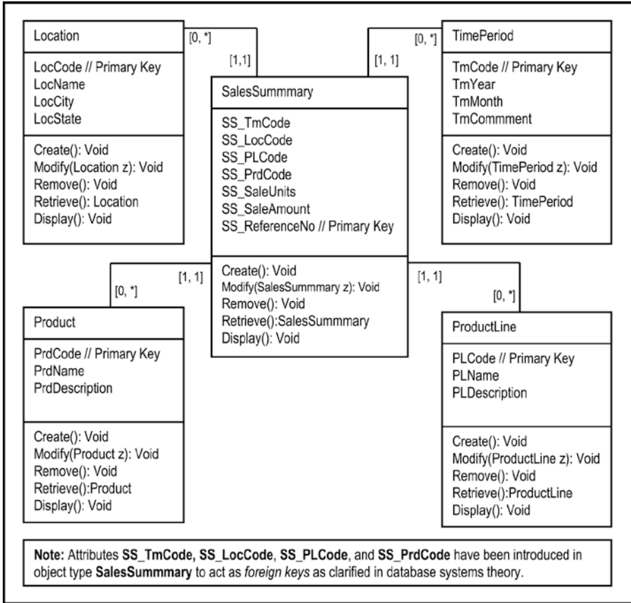
Figure A5-6. ORD for Tracking Sales Summary for a Large Marketing Company
