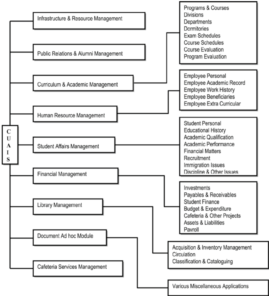
Figure A3-3. Partial Information Topology Chart for the CUAIS Project
